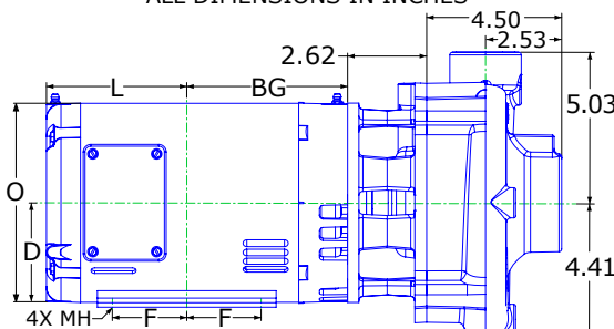
DRAWING DEPICTS JM145 3PHASE TEFC MOTOR ALL DIMENSIONS IN INCHES
