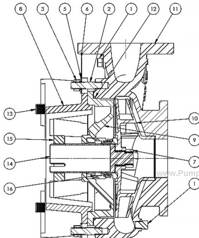
SECTION VIEW SCALE 1:1.25
