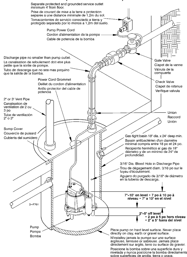
Figure 1. Typical Installation • Installation Type
