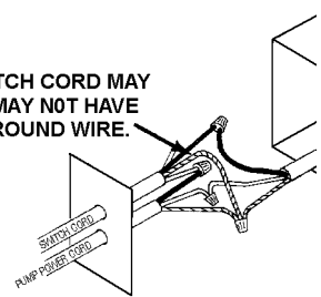
Figure 5 230V Installation
