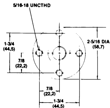
PULLEY MOUNTING PLATE USED ON MODEL 18930-0000
