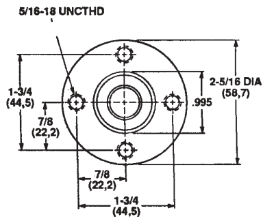
PULLEY MOUNTING PLATE USED ON MODEL 18830-0000
