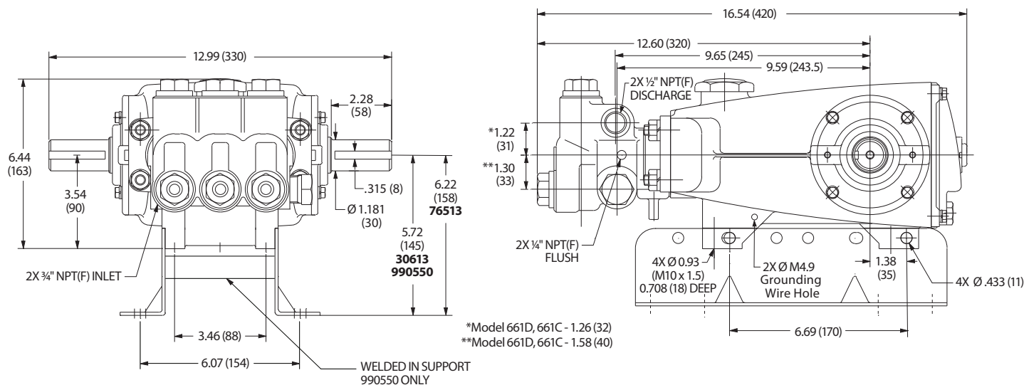
Models 660, 661C, 661D
