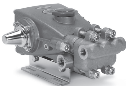
Model 240 Shown (Shaft protector and mounting rails sold separately)
