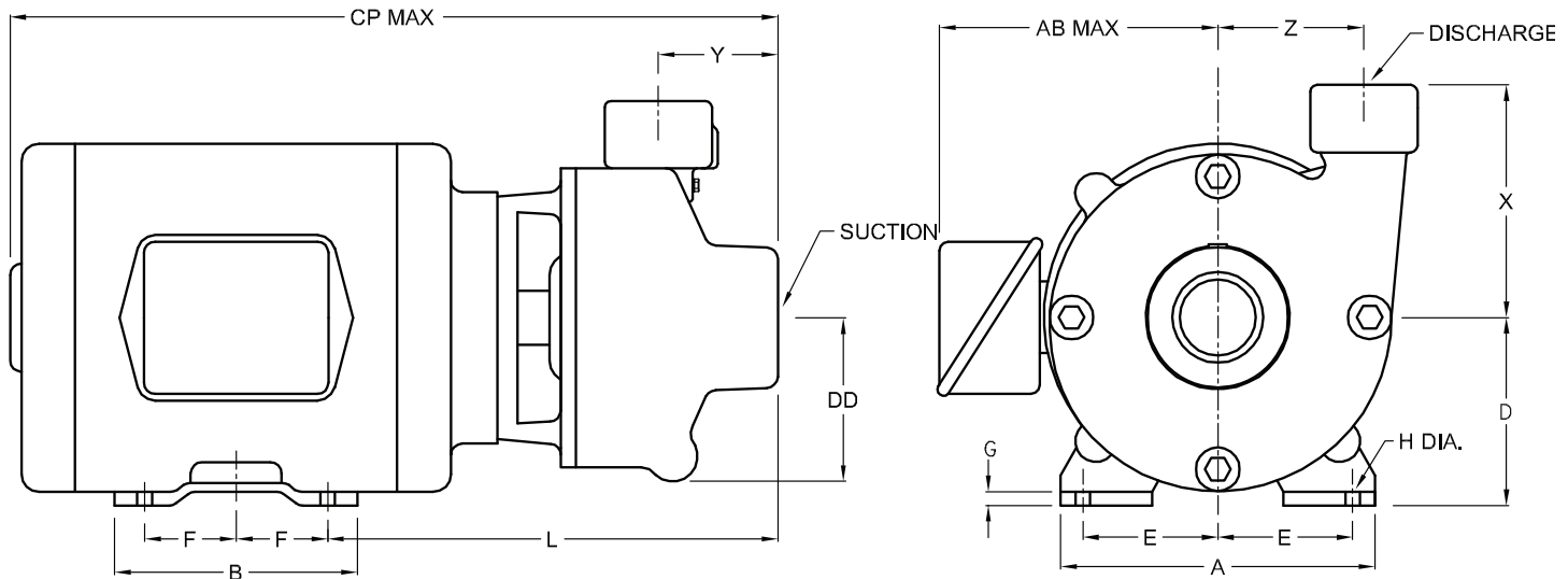
DIMENSIONS IN INCHES
