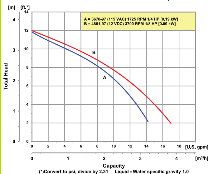
Performance of Bronze Marine Pumps
