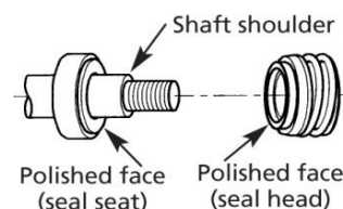
Figure 1 – Seal Replacement
