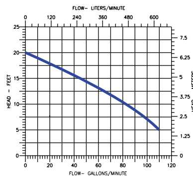
10S SERIES PUMP PERFORMANCE CURVE
