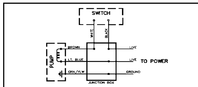
Figure C — Direct Wire Installation
