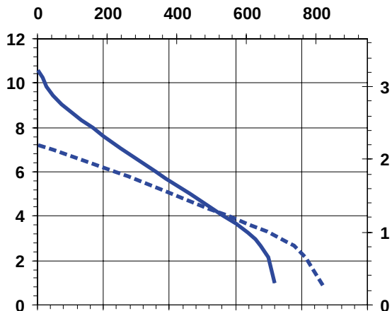
FLOW - LITERS/HOUR
