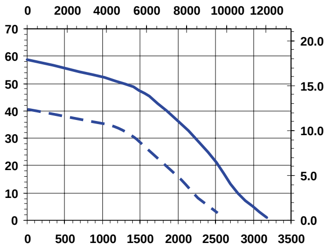
FLOW - LITERS/HOUR
