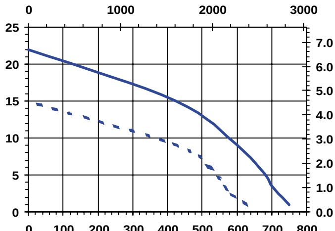
FLOW - LITERS/HOUR
