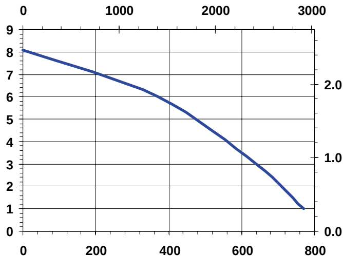
FLOW - LITERS/HOUR
