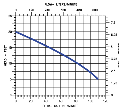
10S SERIES PUMP PERFORMANCE CURVE
