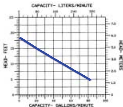
9S SERIES PUMP PERFORMANCE CURVE
