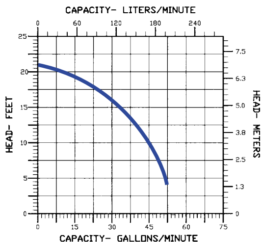
8E SERIES PUMP PERFORMANCE CURVE
