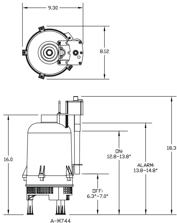
OVERALL DIMENSIONS W/LEG KIT
