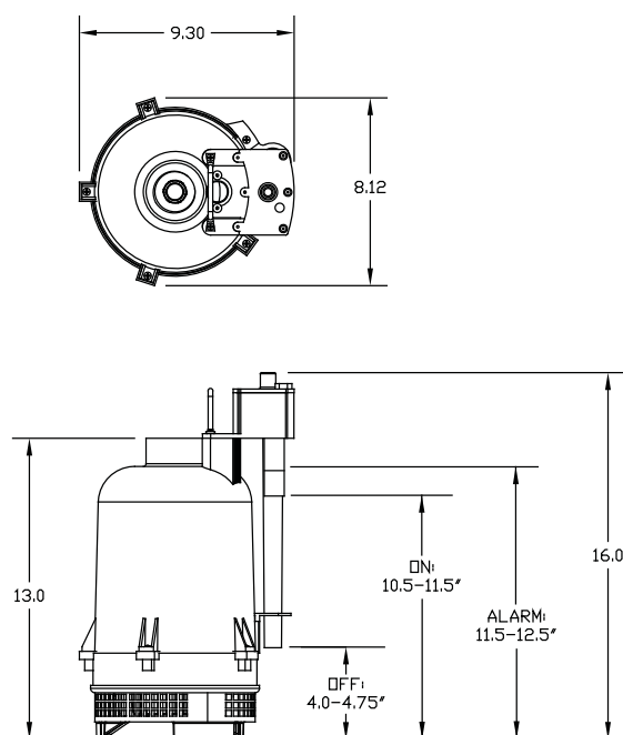
OVERALL DIMENSIONS W/O LEG KIT
