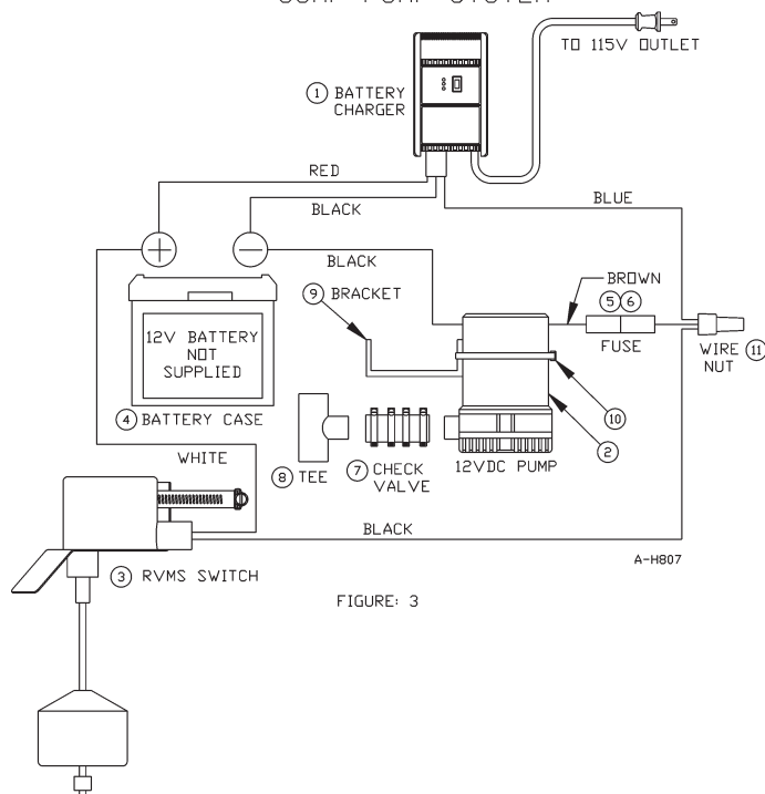
12 VOLT BATTERY BACKUP SUMP PUMP SYSTEM
