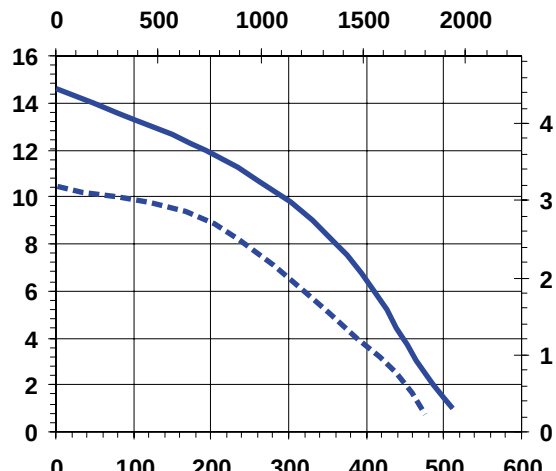
FLOW - LITERS/HOUR
