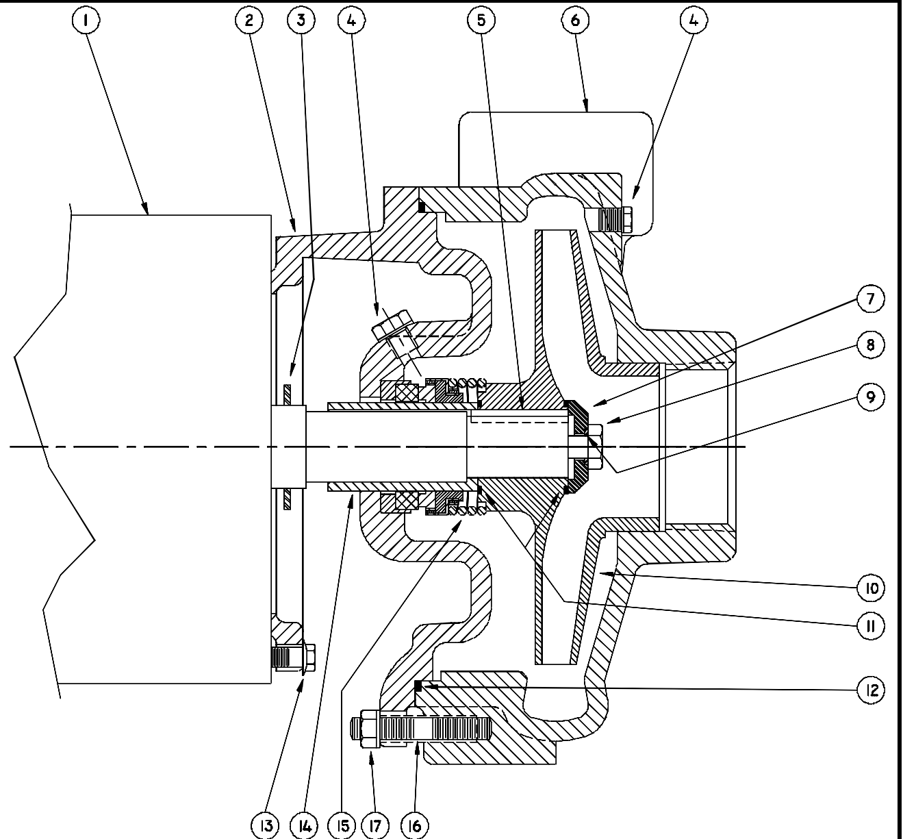
SERIES: GA6-1-1/2 & GA6-2 CENTRIFUGAL PUMPS
